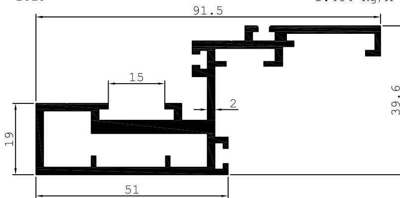
1019 PANNEL FRAME 1.464 Kg/M
