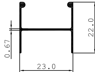
1/2" THREE TRACK BULB
