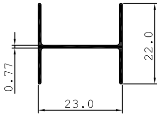
1/2" THREE TRACK PLAIN
