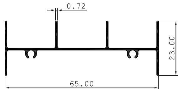
1" TWO TRACK BOTTOM
