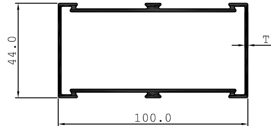
100 X 44 DOUBLE PARTITION
