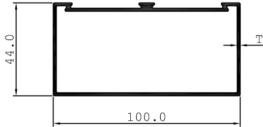
100 X 44 SINGLE PARTITION
