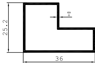
1 1/2 X 1 L TUBE
